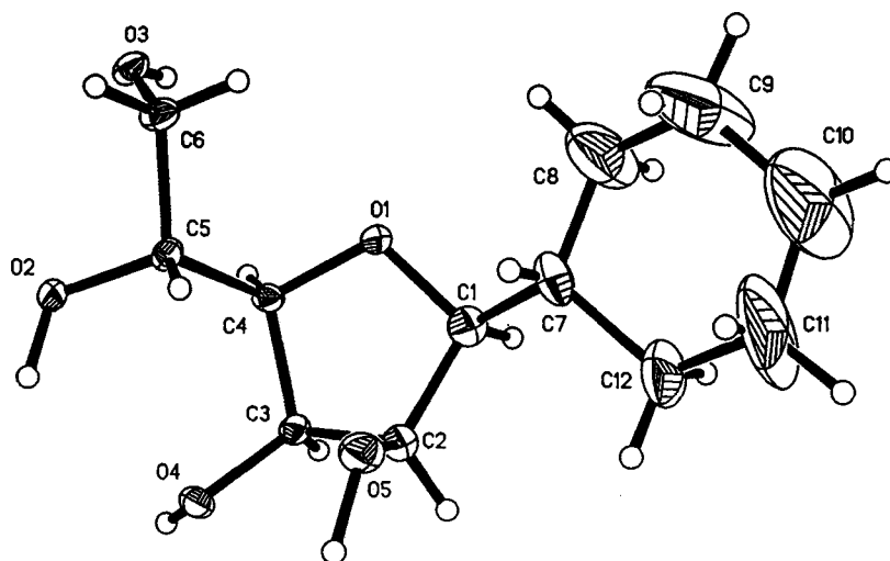
Fig. 2. X-Ray structure of 13. Arbitrary numbering.
